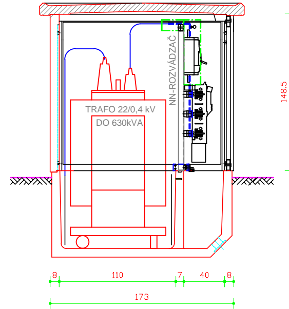
REZ "D-D"
