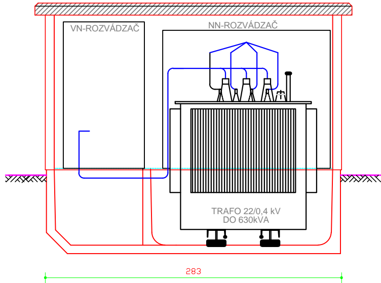
REZ "A-A"
