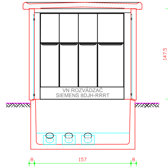
REZ "D-D"
