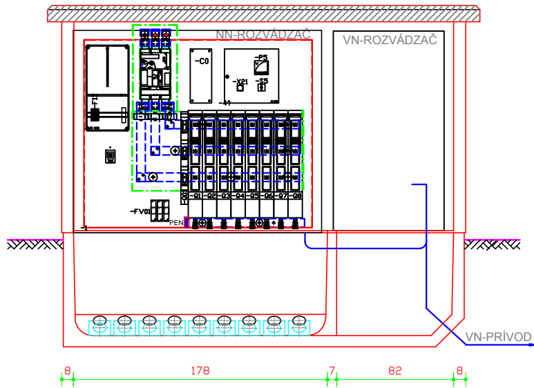
REZ "C-C"
